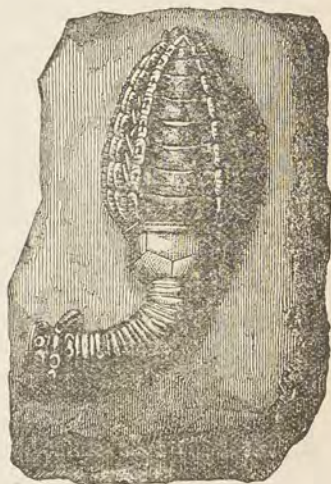
CUPRESSOCRINUS CRASSUS. (Old Red Sandstone.)
